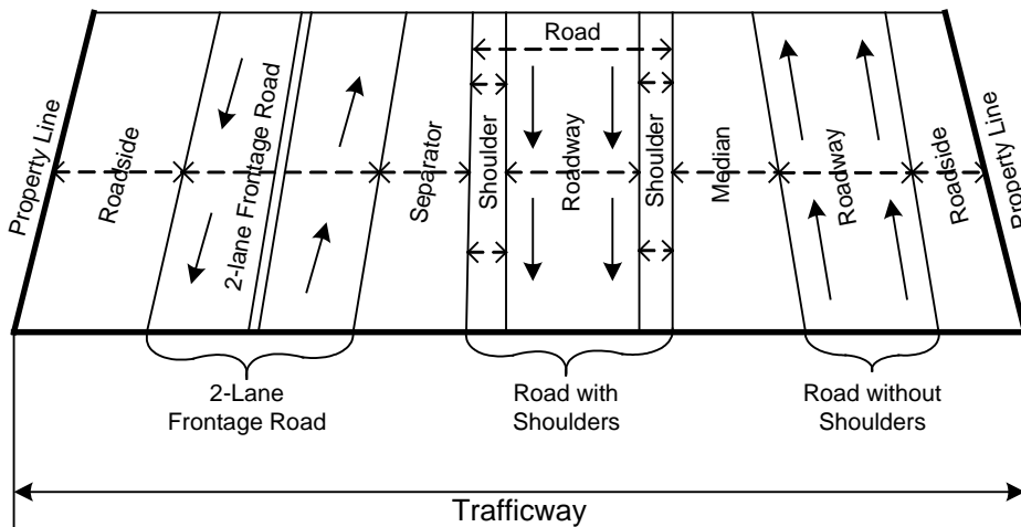
Trafficway with Frontage Road
